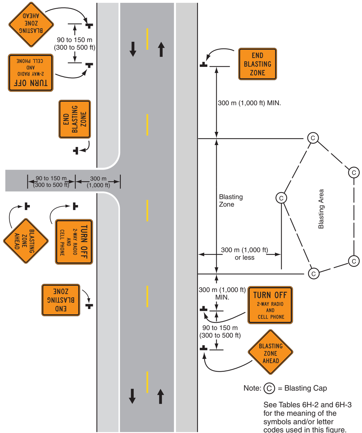
Typical Application 2
