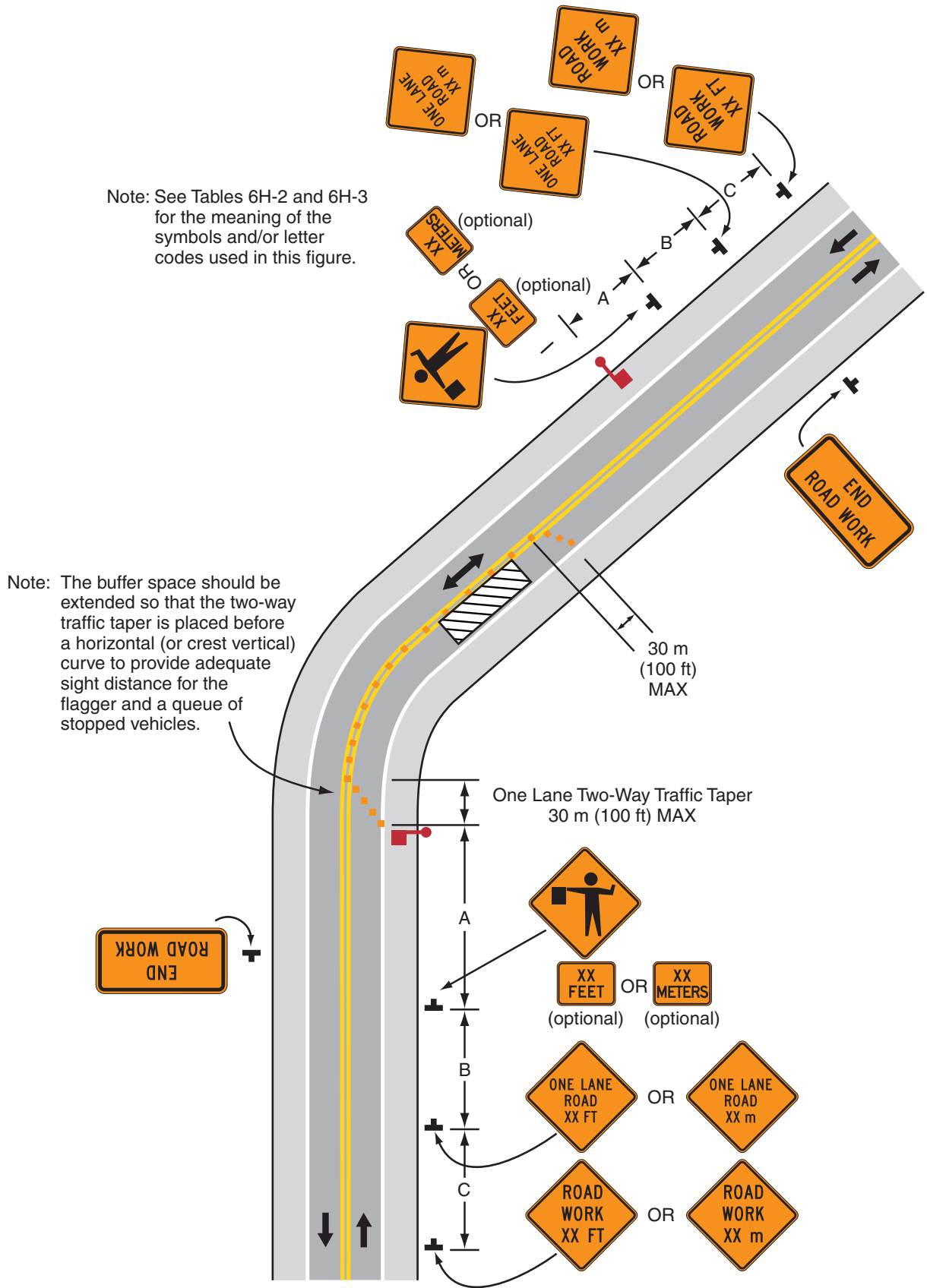
Typical Application 10
