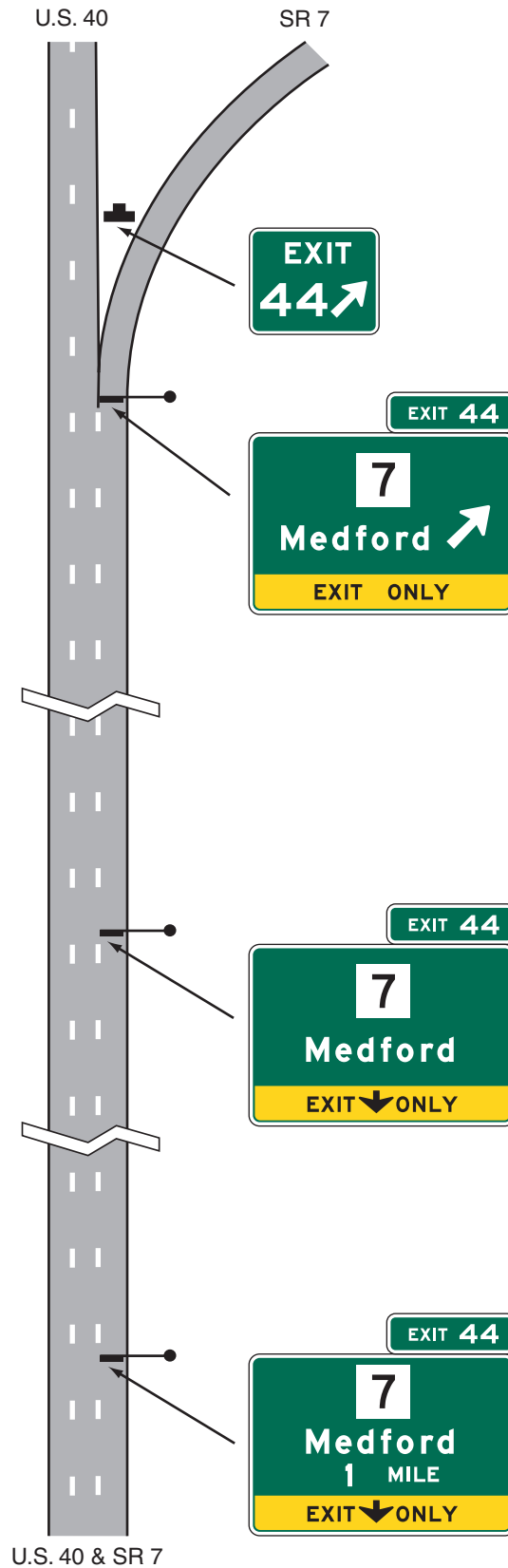
Figure 2E-10. EXIT ONLY Panels for Right Lane Dropped at an Interchange
