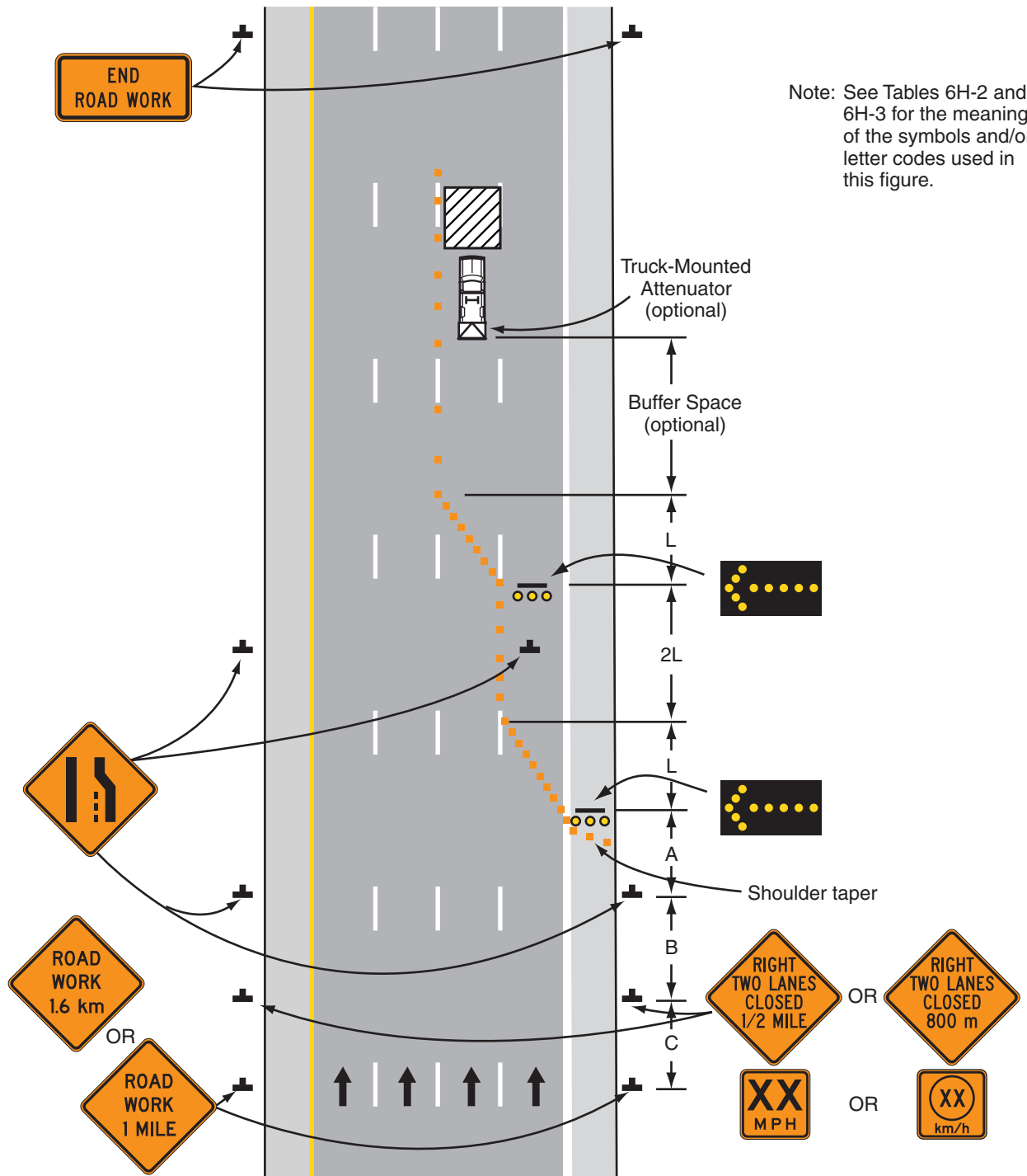
Typical Application 37
