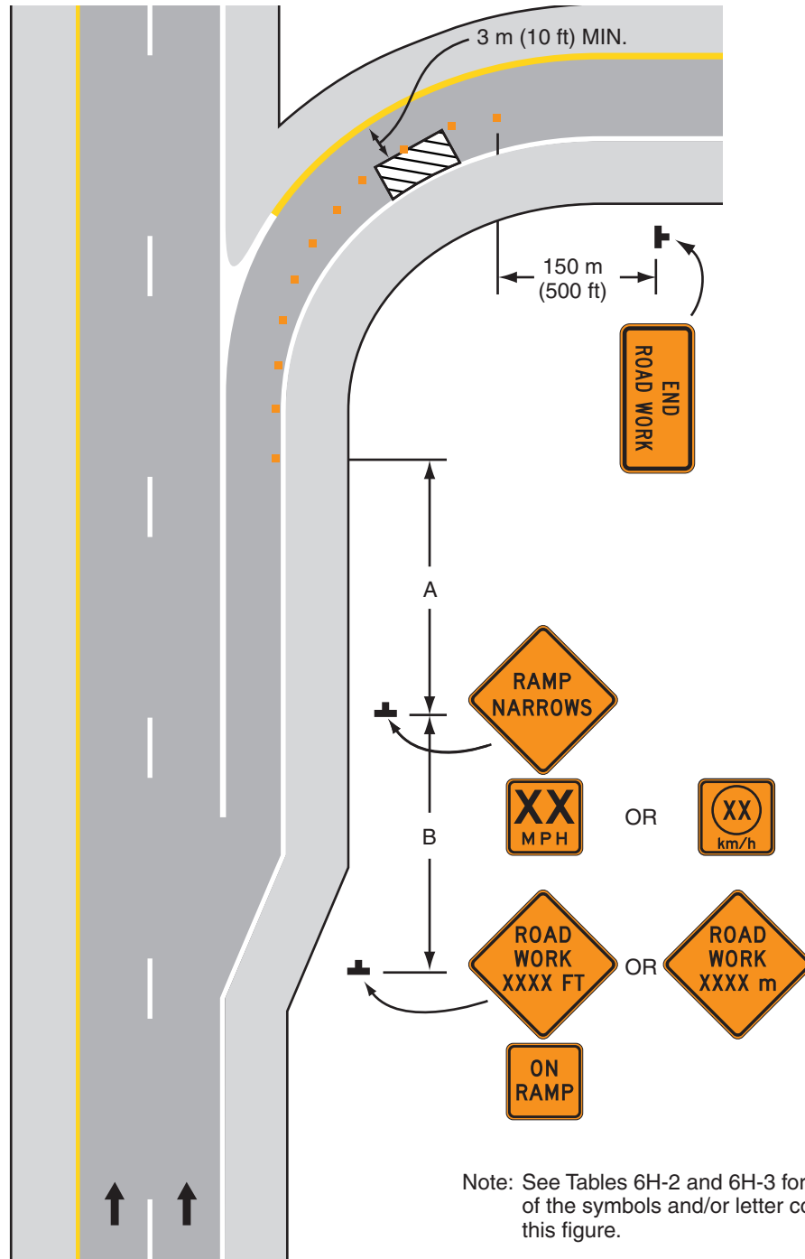
Typical Application 43
