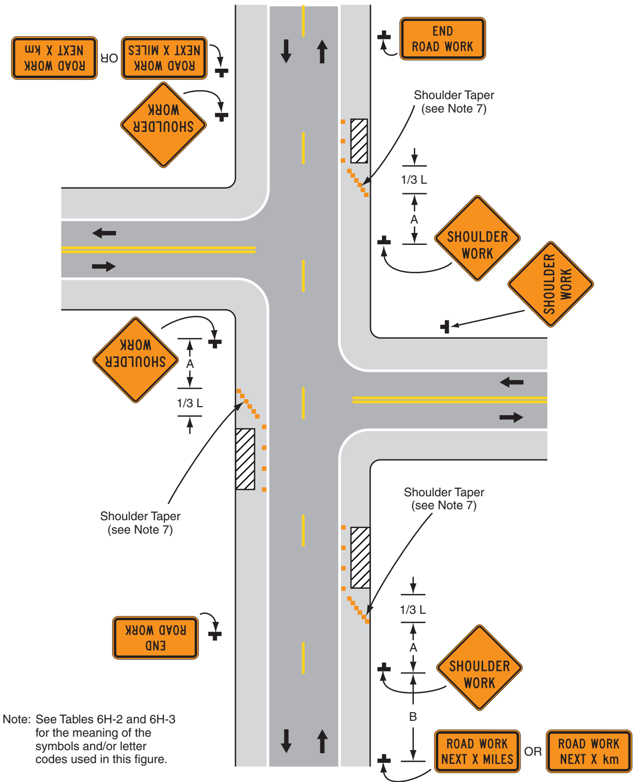
Typical Application 3
