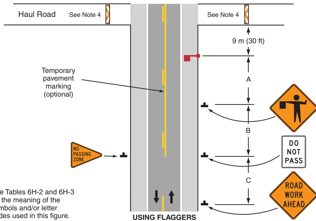
Typical Application 14
