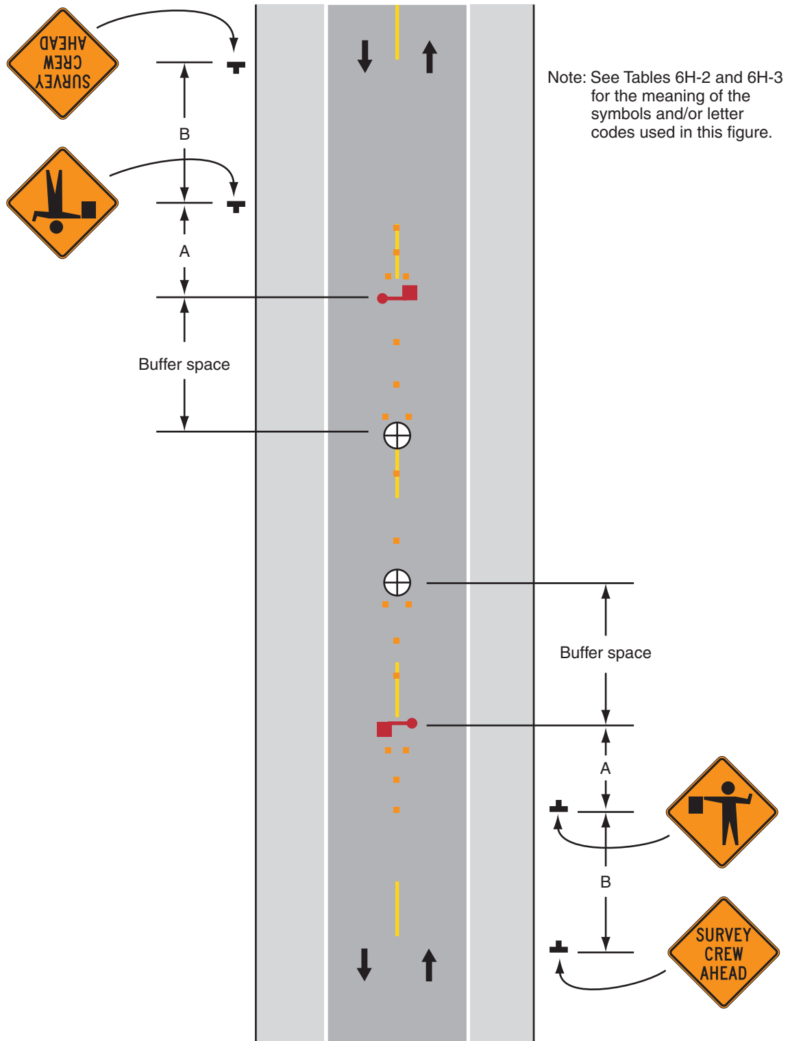
Typical Application 16
