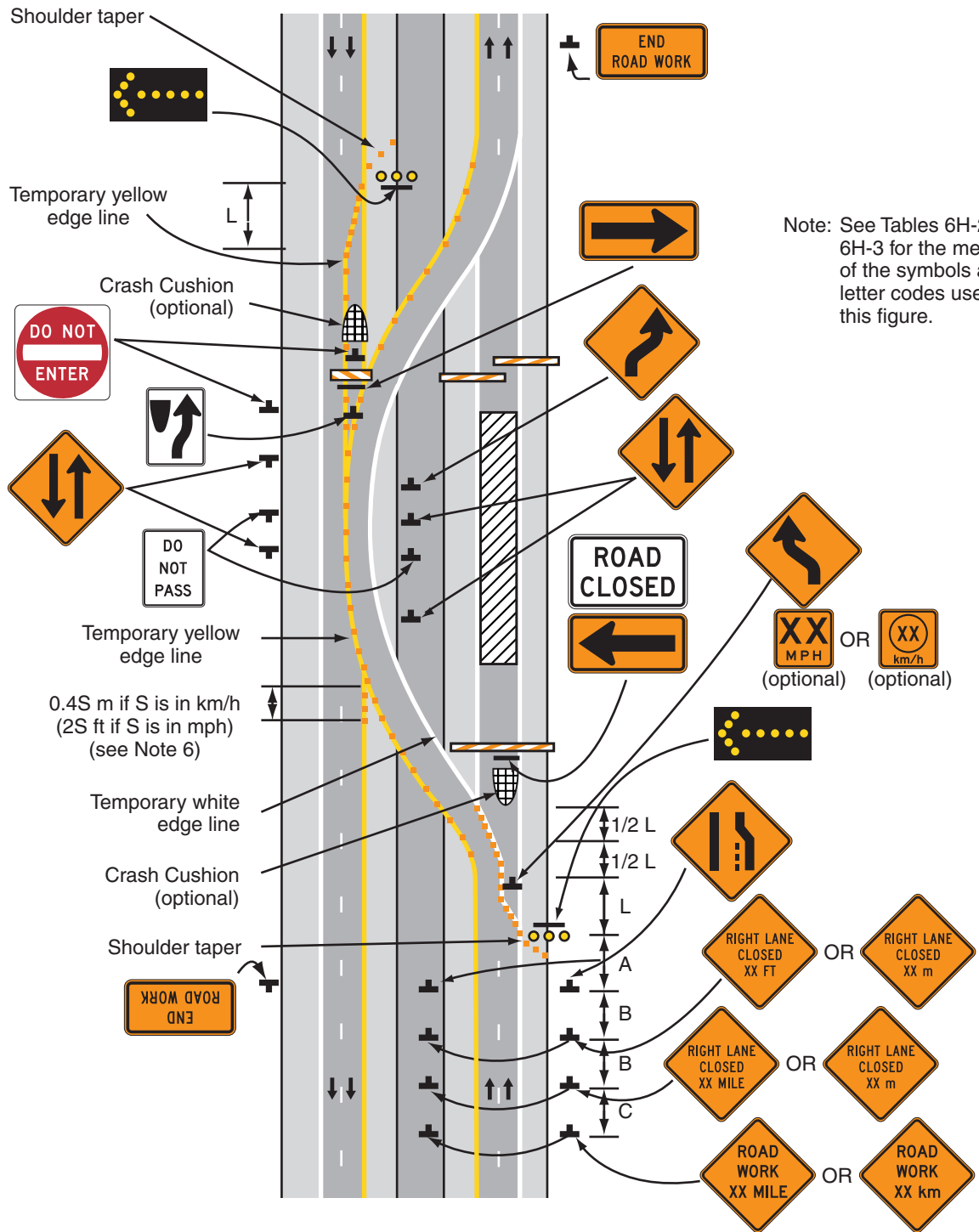
Typical Application 39
