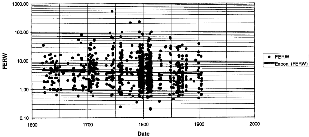
Figure 3-39. Fractional Exchange Ratio Favoring the Winner versus Date for the BWSHALL Data Base
