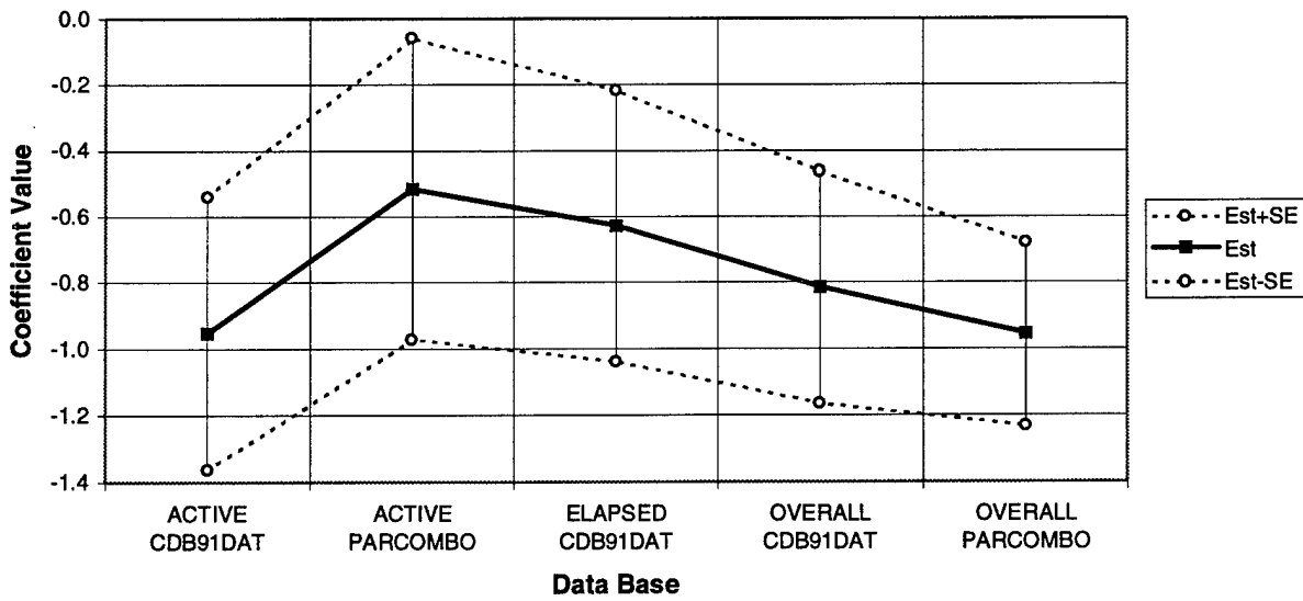
Figure 4-6. Constant Term for Regression of InCY using Various Data Bases
