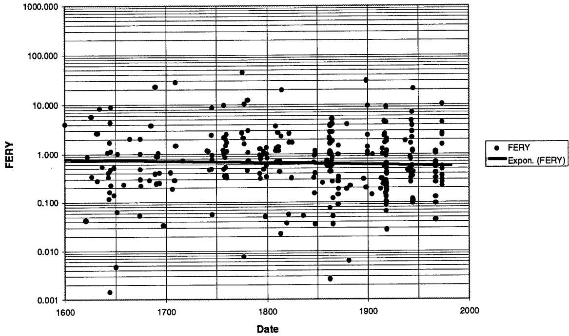
Figure 3-15. Fractional Exchange Ratio Favoring the Defender versus Date for the CDB91DAT Data Base
