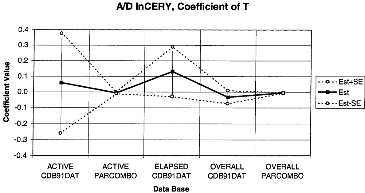
Figure 4-12. Coefficient of T for Regression of lnCERY using Various Data Bases
