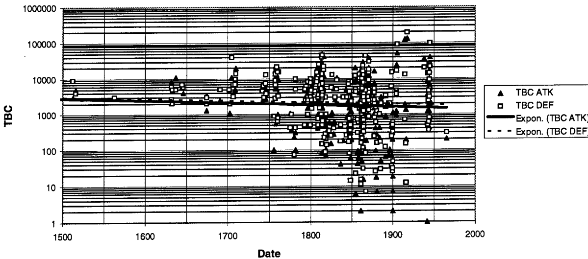
Figure 3-10. Attacker and Defender TBC versus Date for the PARCOMBO Data Base
