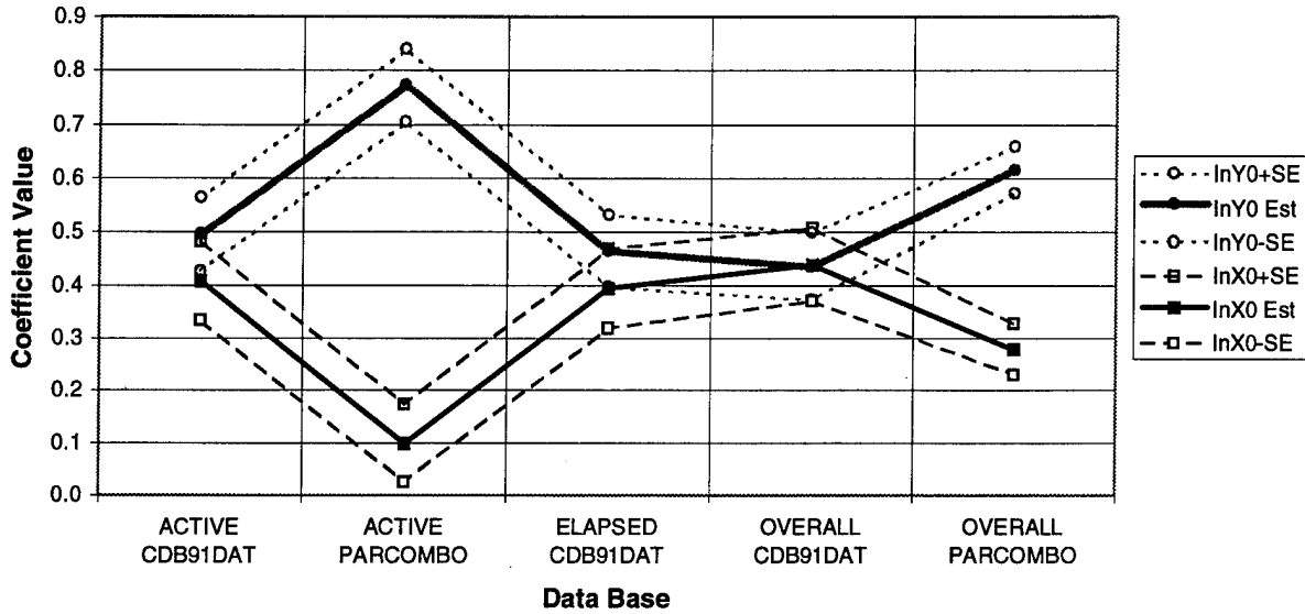
Figure 4-7. Coefficients of lnX0 and lnY0 for Regression of lnCY using Various Data Bases
