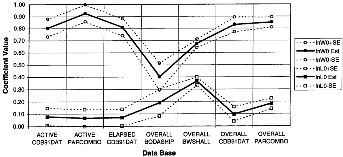
Figure 4-16. Coefficients of InW0 and InL0 for Regression of InCW using Various Data Bases
