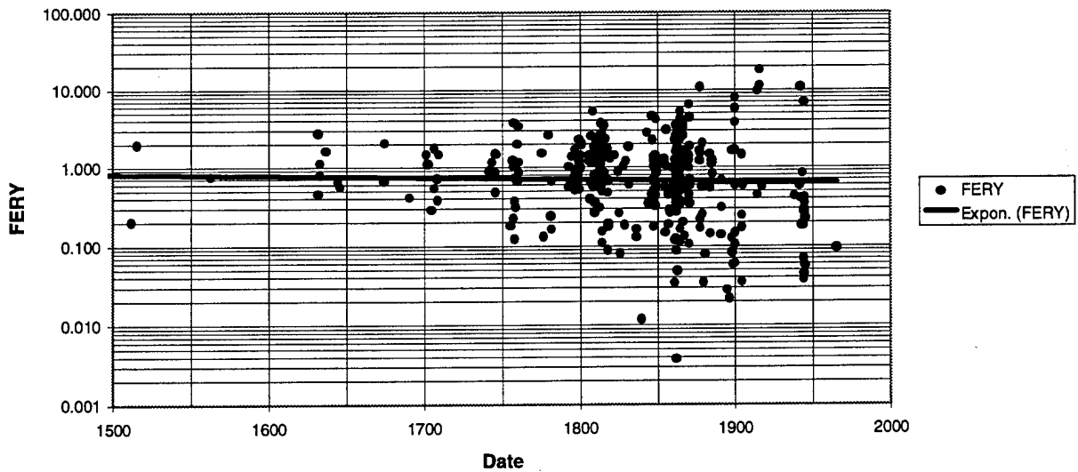
Figure 3-16. Fractional Exchange Ratio Favoring the Defender versus Date for the PARCOMBO Data Base
