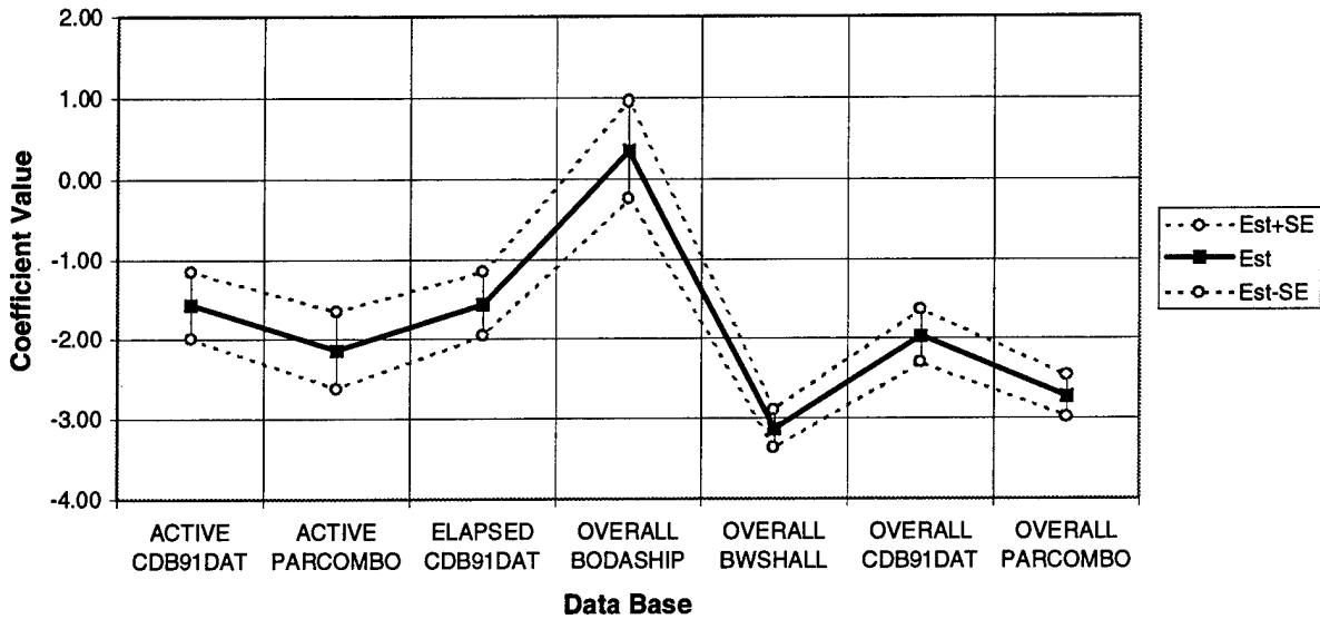
Figure 4-15. Constant Term for Regression of InCW using Various Data Bases
