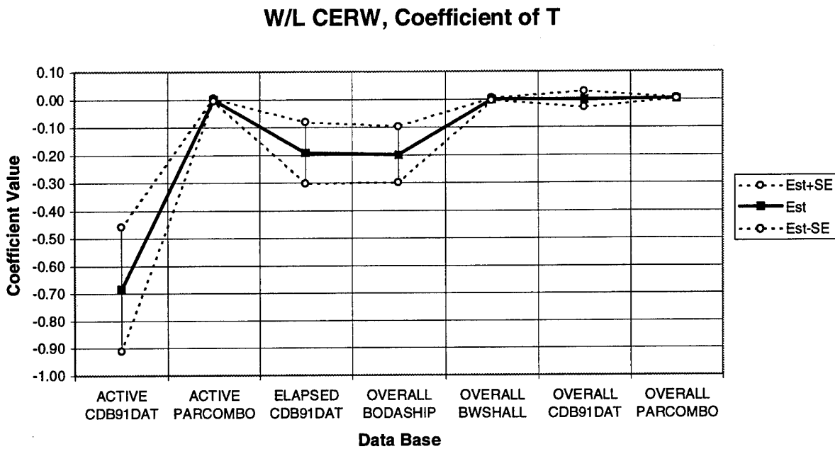
Figure 4-25. Coefficient of T for Regression of lnCERW using Various Data Bases
