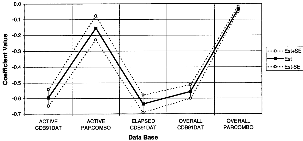
Figure 4-5. Coefficient of D for Regression of InCX using Various Data Bases
