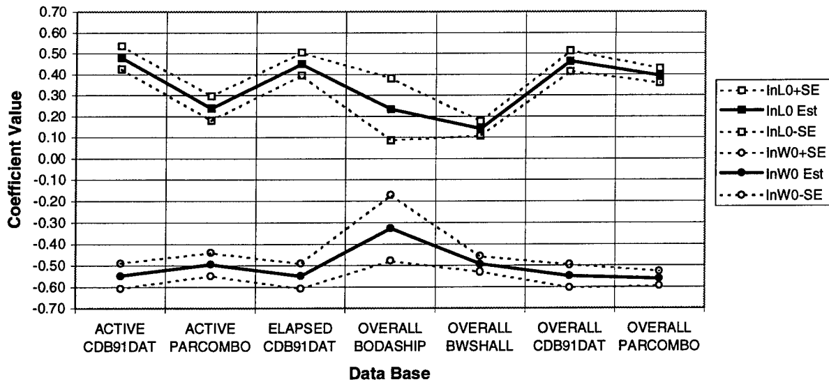
Figure 4-24. Coefficients of InW0 and InL0 for Regression of InCERW using Various Data Bases
