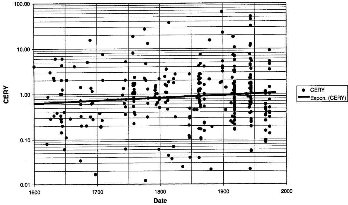
Figure 3-11. Casualty Exchange Ratio Favoring the Defender versus Date for the CDB91DAT Data Base
