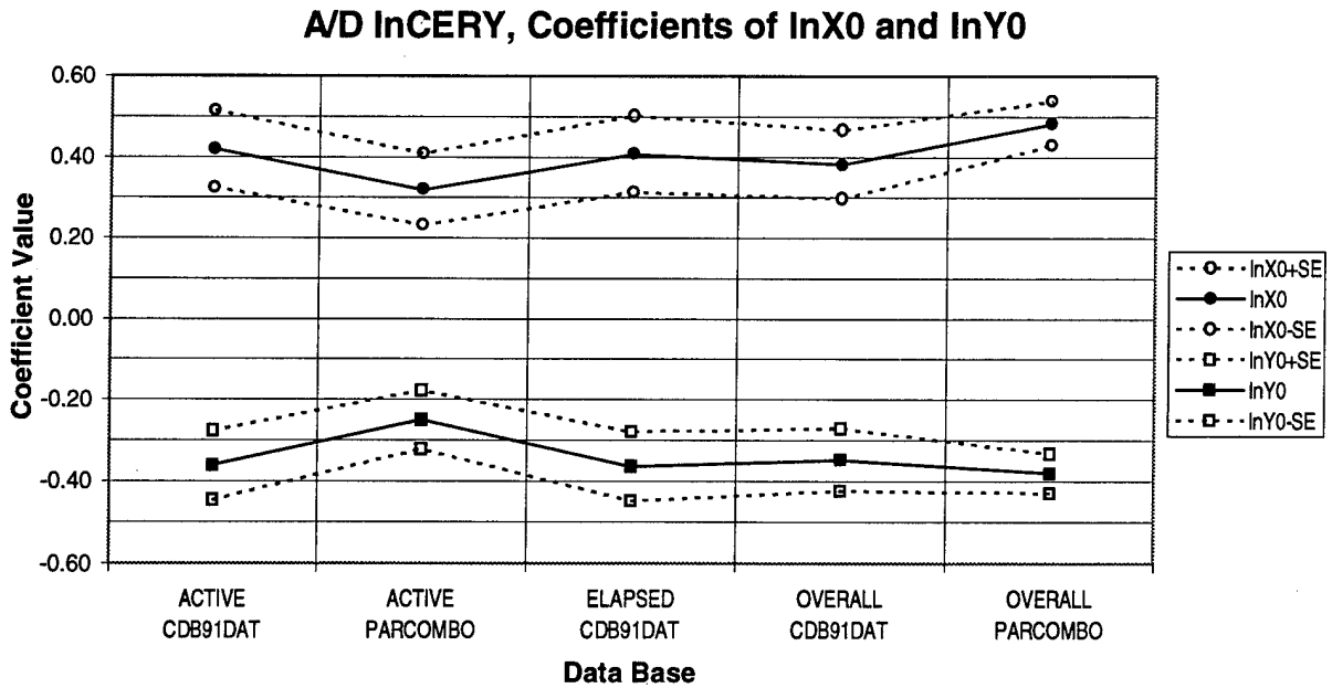
Figure 4-11. Coefficients of lnX0 and lnY0 for Regression of lnCERY using Various Data Bases
