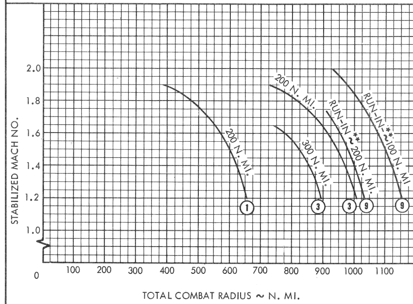
EFFECT OF MACH NUMBER ON COMBAT RADIUS
