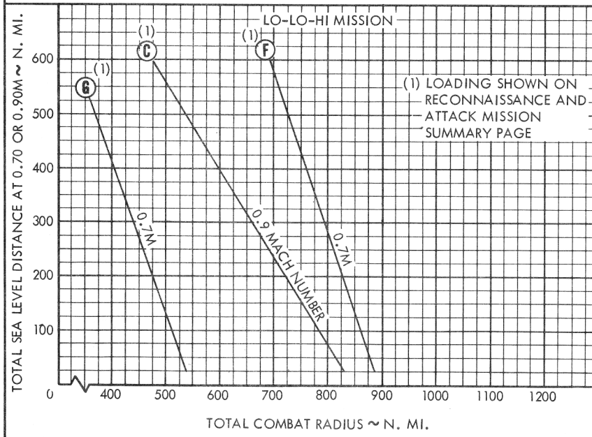
EFFECT OF S. L. DISTANCE ON COMBAT RADIUS
