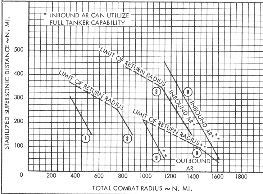
EFFECT OF SUPERSONIC DISTANCE ON COMBAT RADIUS
