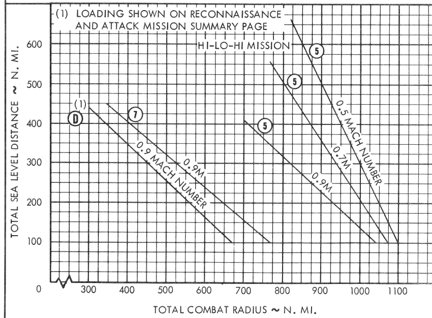
EFFECT OF MACH NUMBER ON COMBAT RADIUS N. MI.
