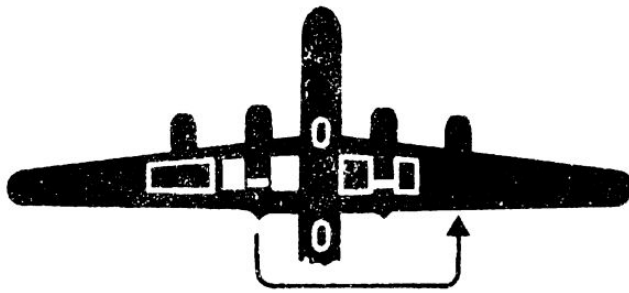
DESIRED TRANSFER—NO. 2 TANK TO ENG. NO. 4 TANK
