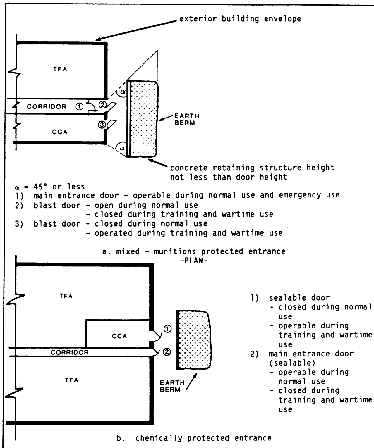
Figure 2 Entrance Arrangements
