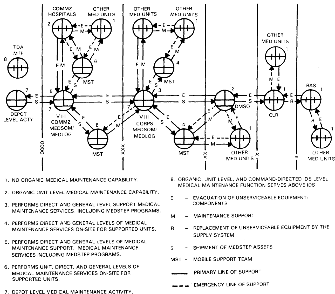
Figure 1-2. Medical maintenance flow.
