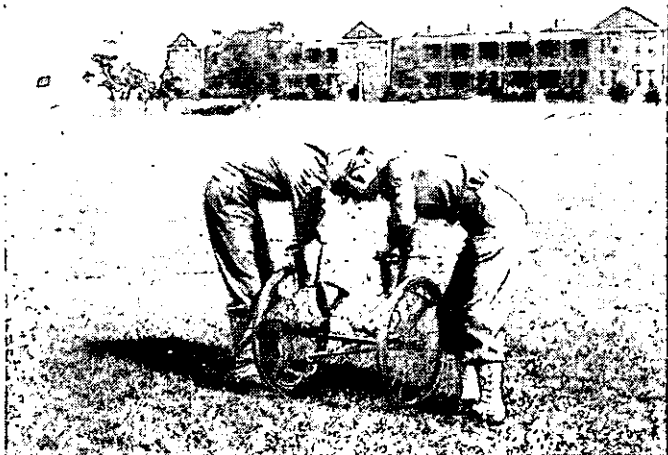
FIGURE 120.—Opening carrier, third step.
