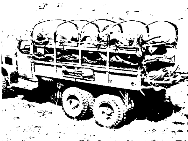
Figure 184. The 2 1/2 ton truck loaded with eighteen litters.
