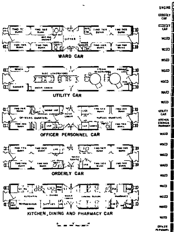
Figure 197. Plan of standard hospital train.
