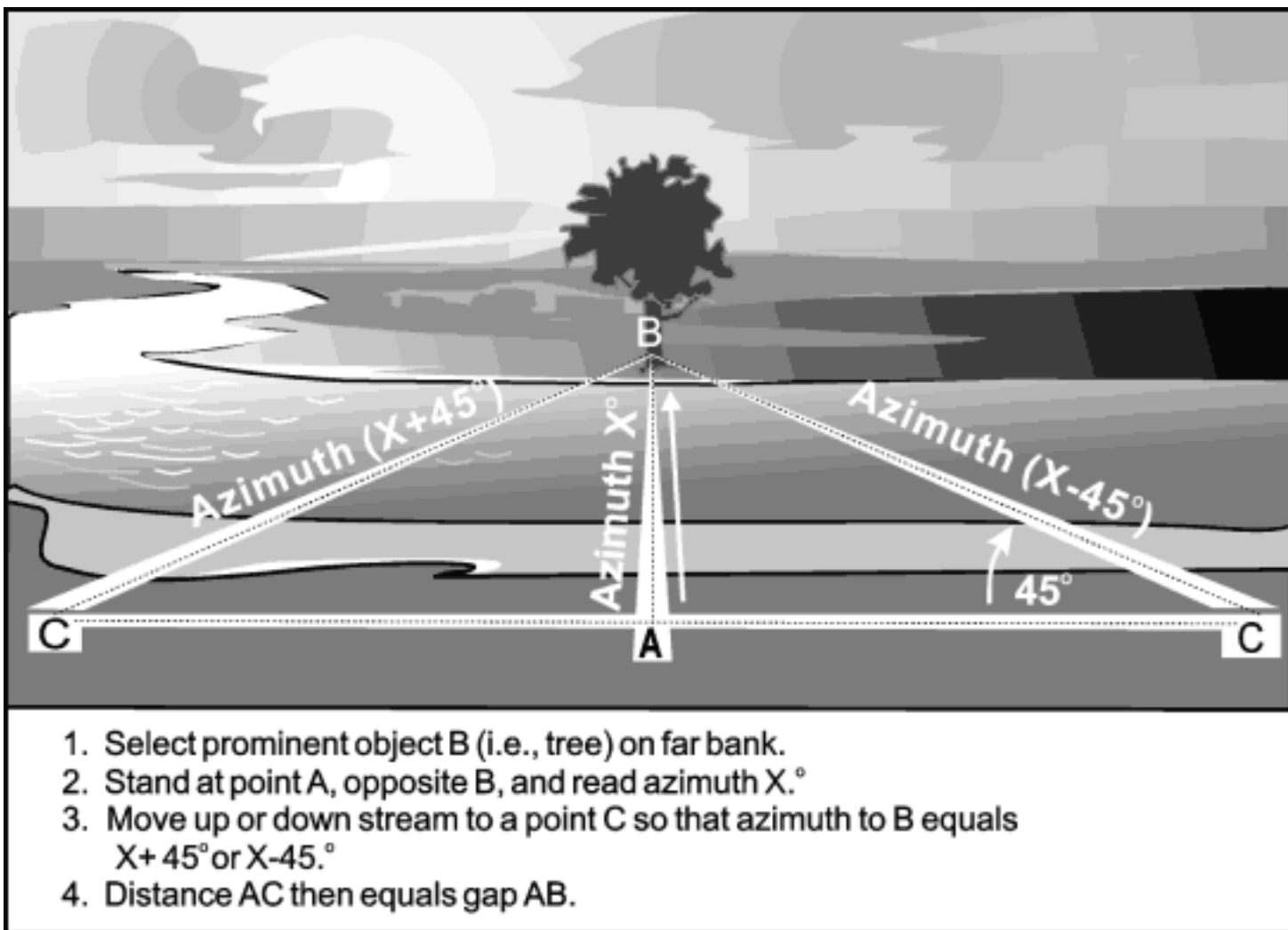
Figure 9-4. Measuring stream width with a compass.
