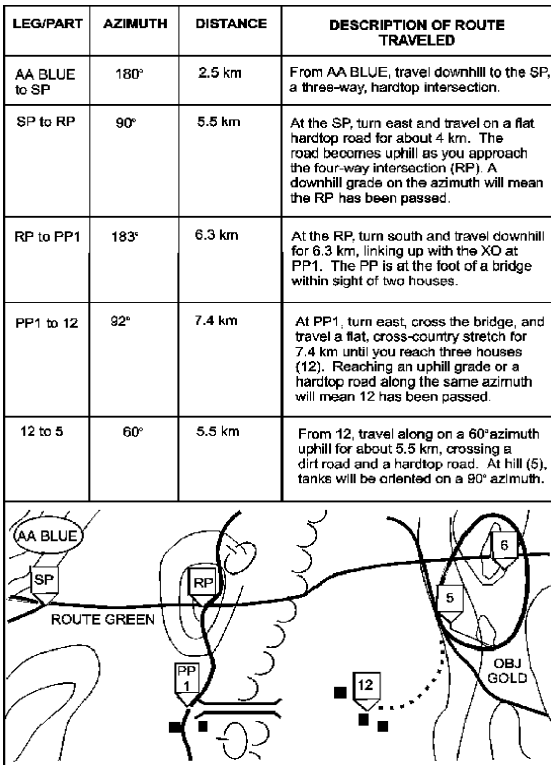
Figure 2-12. Route chart for compass and odometer navigation method.
