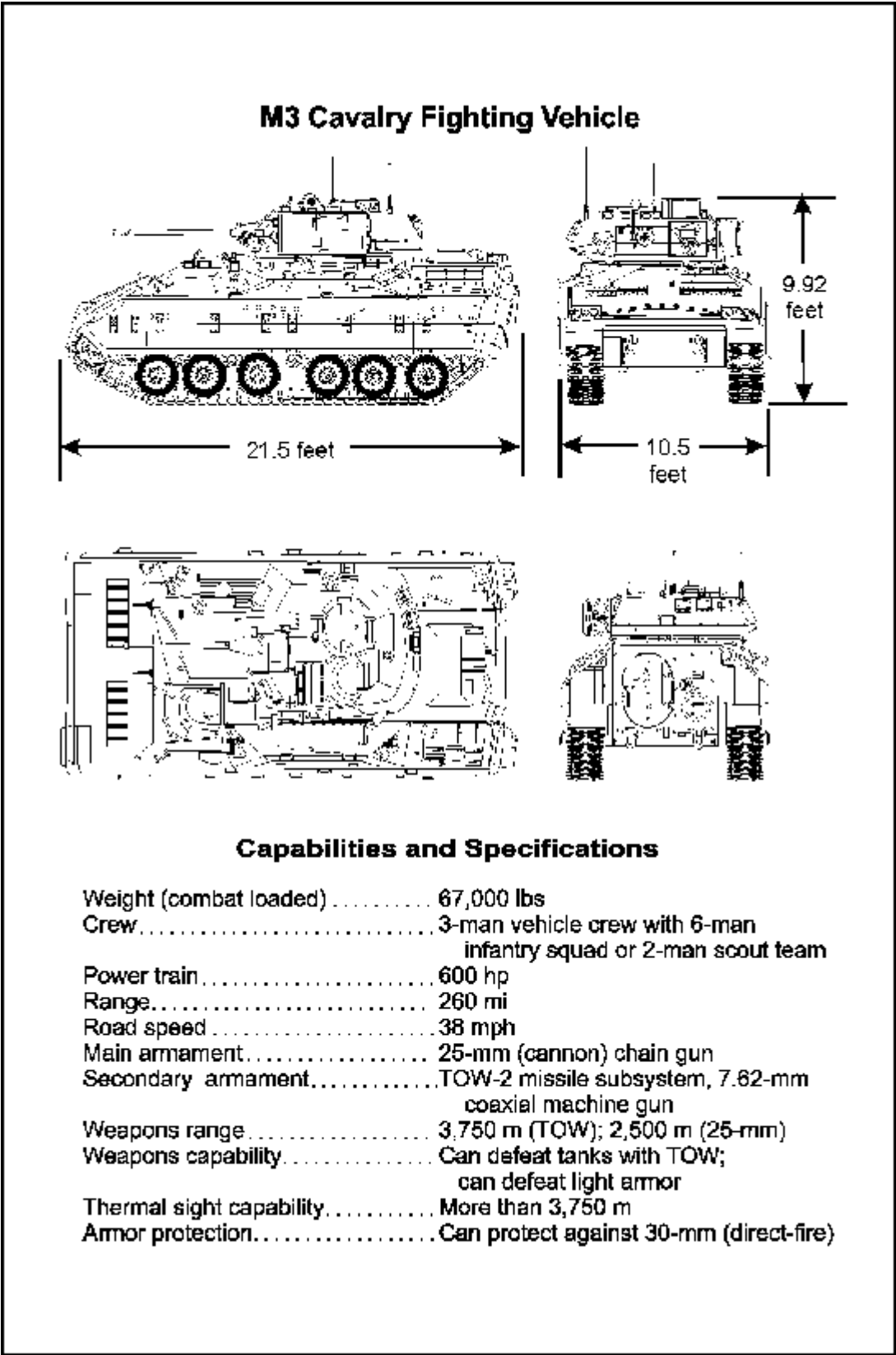
Figure 1-10. M3 CFV characteristics
