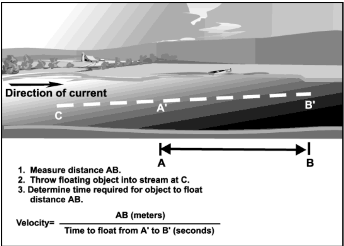
Figure 9-5. Measuring stream velocity.
