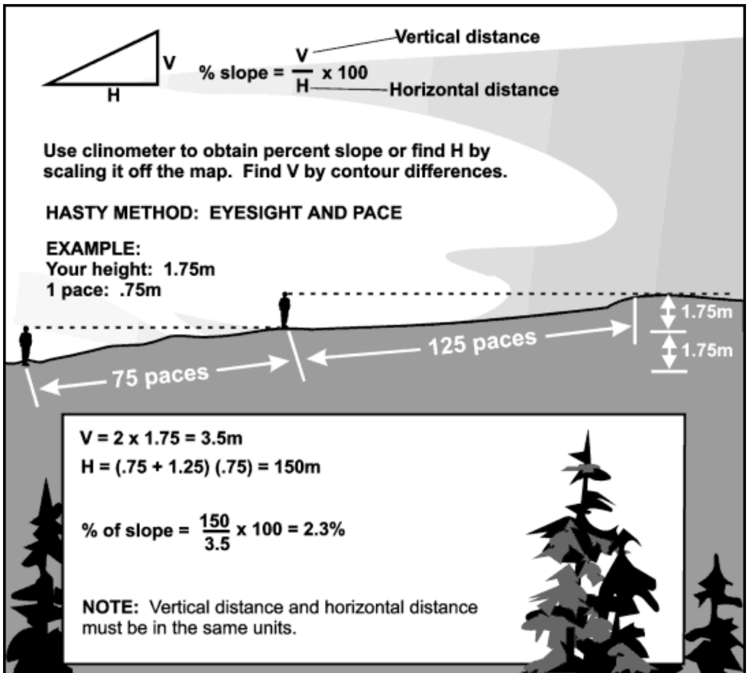
Figure 9-6. Slope computation (road gradient).
