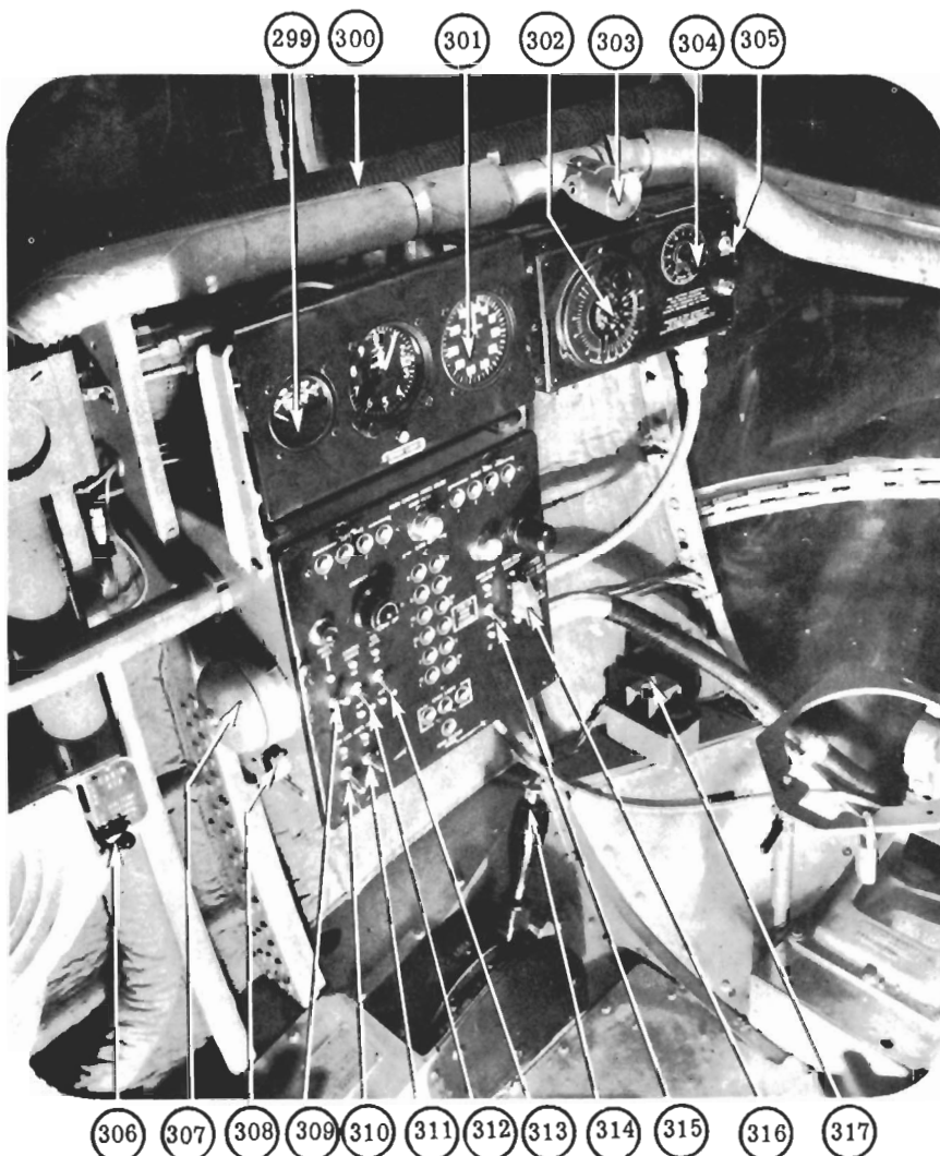
Figure 35 - Bombardier's Compartment (Left Side)
