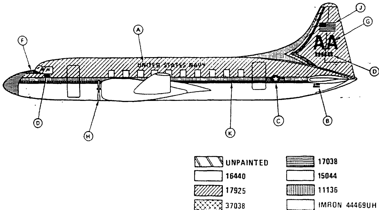
FIGURE D-9. C-131H aircraft marking.
