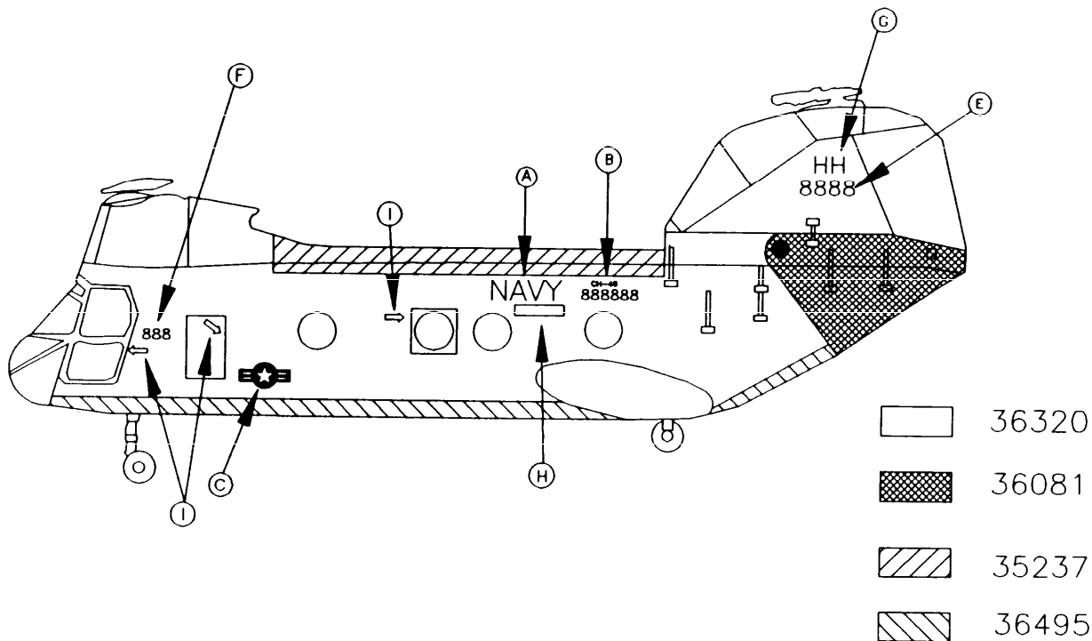
FIGURE C-33. UH-46A/D aircraft marking.
