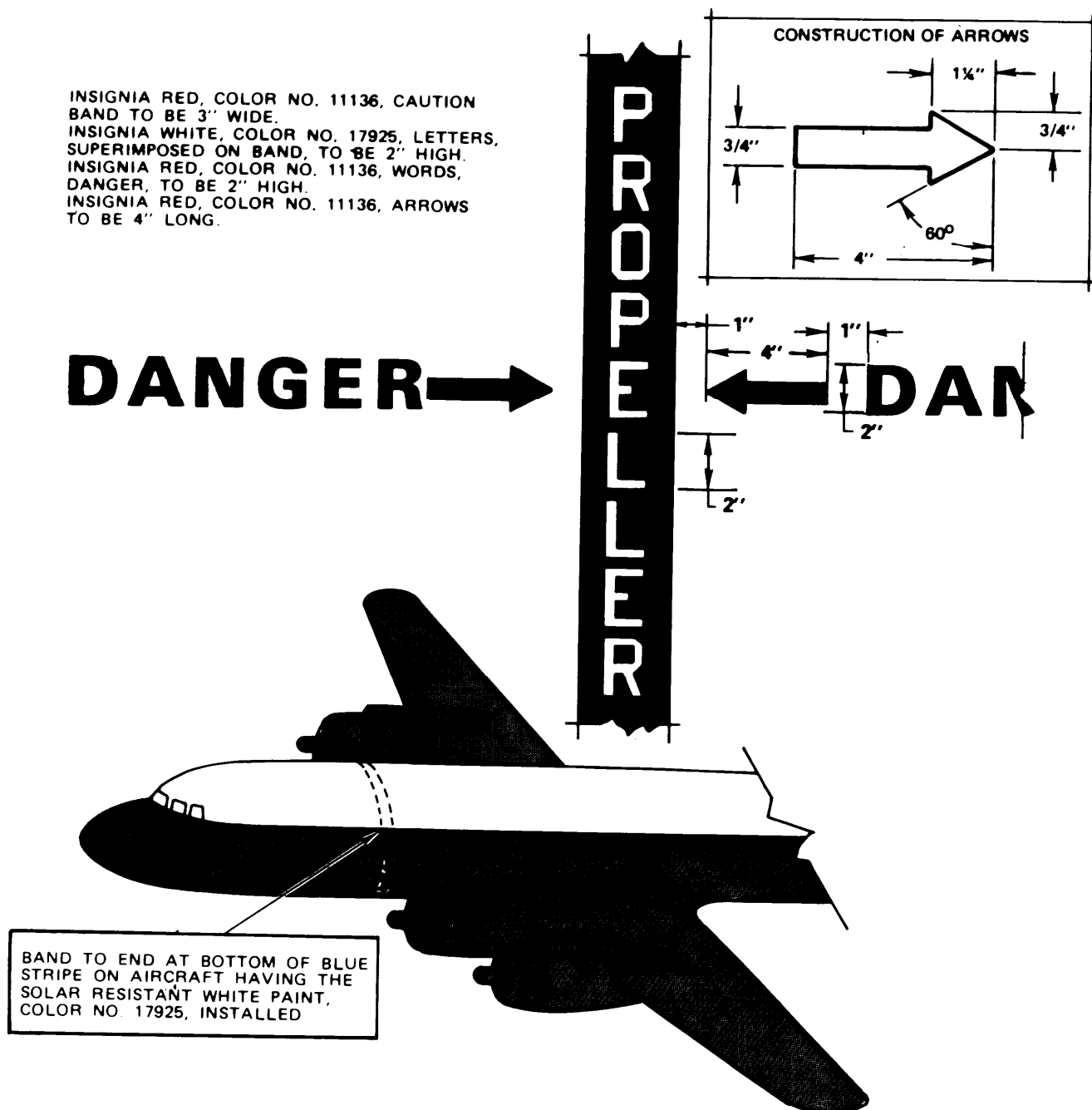
FIGURE A-9. Propeller warning strips and signs.
